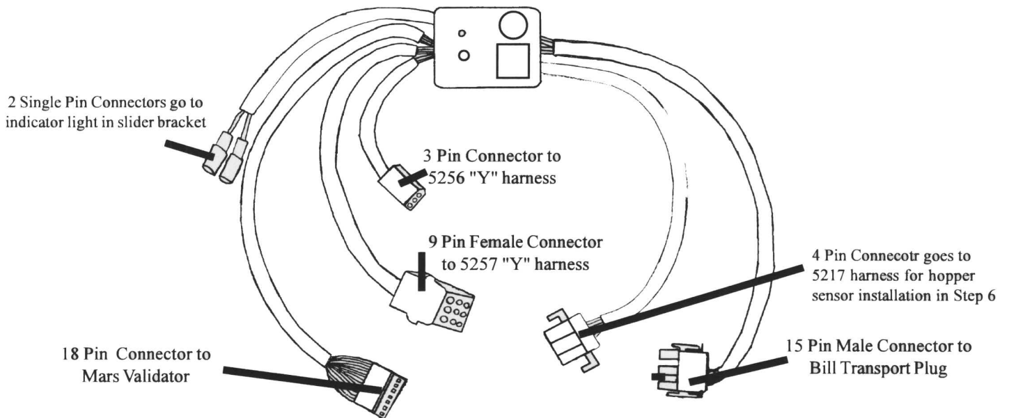
Figure 7 5252 Main Box and Harness Assembly
