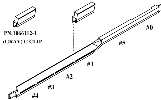
Gage Bar Clip Location
