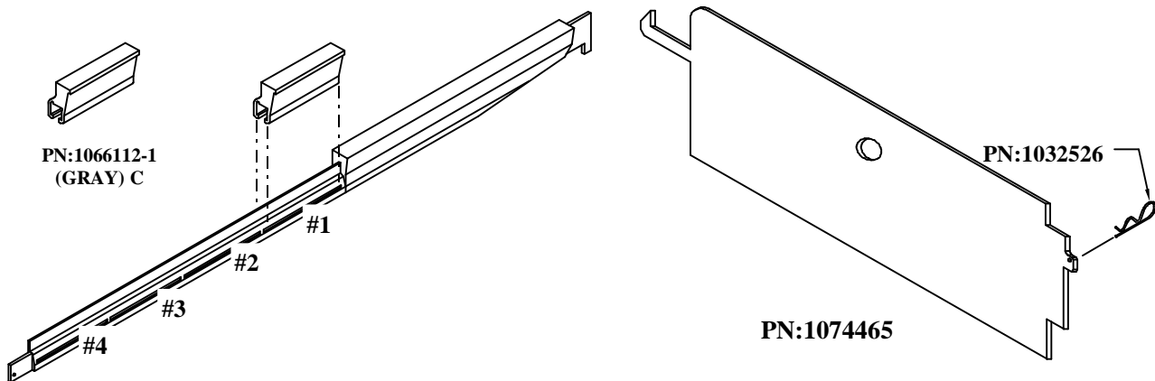
Gage Bar Clip Location
