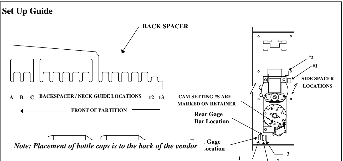
GAGE BAR LOCATIONS
